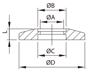
Bored Flange
