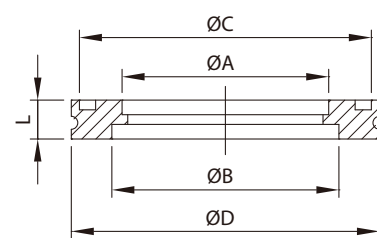
Weld Flange
