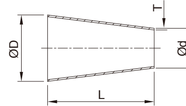
Concentric Reducer
