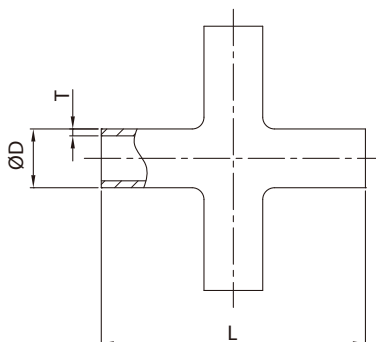
9W LONG CROSS WELD END
