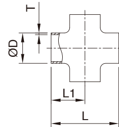
Cross
