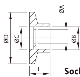
Socket Weld Flange
