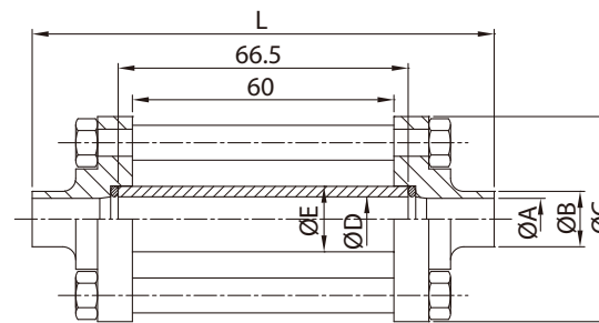
3A/BS WELD END SIGHT GLASS
