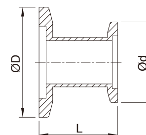
Straight Reducer
