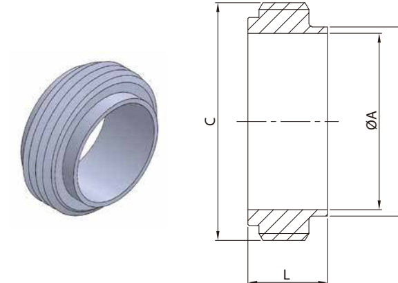
IDF-15 WELDING MALE
