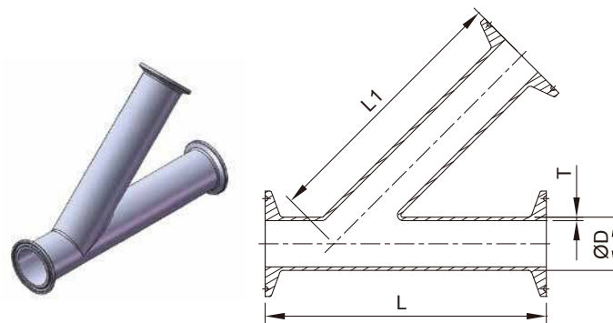
28AMP 45° CLAMP EQUAL LATERALS
