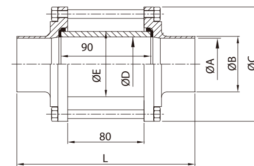
SMS WELD END SIGHT GLASS
