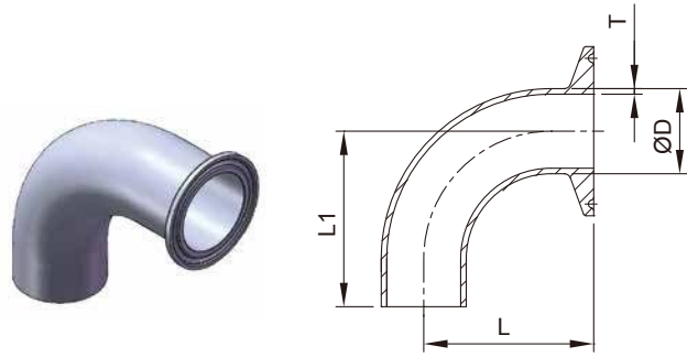
L2CM WELD/CLAMP 90° ELBOW
