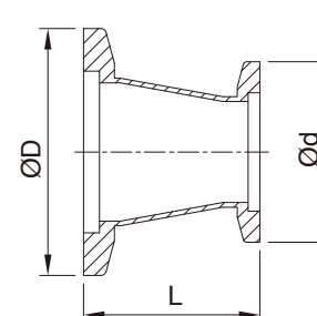
Conical Reducer
