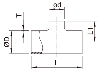
Reducing Tee
