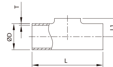
7WWO SHORT EQUAL PULL WITHOUT STRAIGHT WELD TEE
