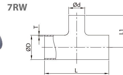
REDUCING TEE/REDUCING TEE
