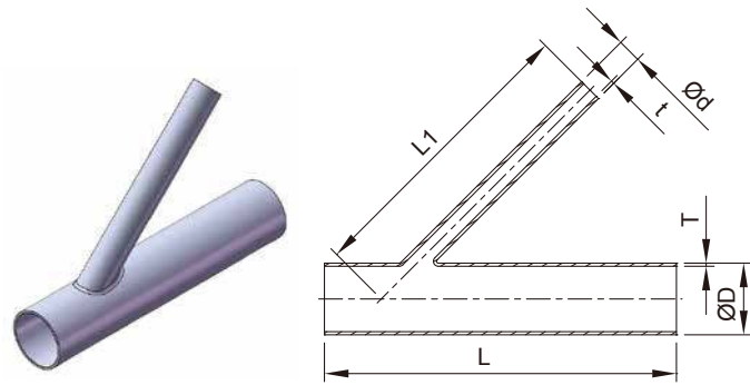
45° WELD REDUCING LATERALS
