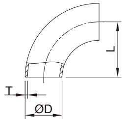
90° Short Elbow
