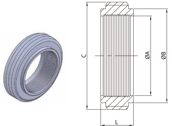
IDF-15R RECESSLESS MALE
